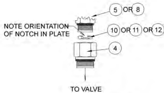
ORIFICE PLATE INSTALLATION DETAIL
