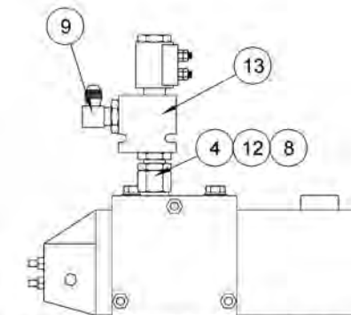
SOLENOID LOCK VALVE INSTALLATION DETAIL
